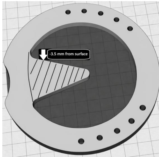
Tabs on Medial Lateral sides of horseshoes (centers on 2 and 10 o'clock )
